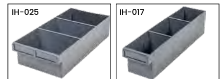
IH-025 Parts Tray Size: (with 3 dividers) 400x200x100mm
